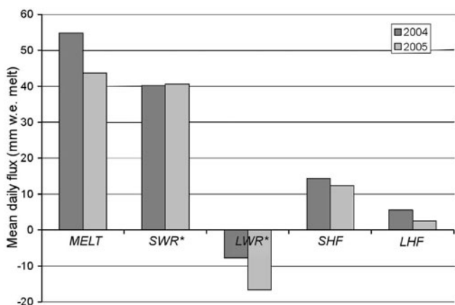
Fig. 3. Modelled mean daily snow surface energy fluxes at the Glacier AWS Site during the January to March periods in 2004 and 2005. SWR* = net shortwave radiation flux; LWR* = net longwave radiation flux; SHF = sensible heat flux; LHF = latent heat flux. All fluxes were converted from W m^{-2} to units of mm w.e. melt using L_f .
