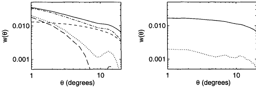
Fig. 1. The solid line in Fig. 1a is the correlation function of the entire APM region. The upper dashed line is dust, and the lower dashed line is the clean APM region (corrected), taken to be the underlying galaxy correlation. The dotted line is the correlation of the full APM region after correcting for dust and stars. The dash-dot line is the sum of the dust and clean lines. In Fig. 1b, the solid and dotted lines are the excess correlation of uncorrected and corrected counts, respectively.
