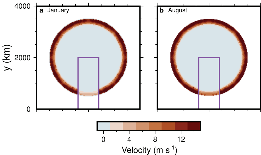
Fig. 5. Comparison of ice sheet surface velocity between the winter and summer for the simulation shown on Figure 3 at 25 000 years. The purple box shows the region that has S_f = 50\% sediment cover. (a) In the winter, the velocity in partially sediment cover is near zero, while the margin regions with continuous cover continue to flow. (b) In the summer, the velocity in partially covered areas increases as a result of the input of water.
