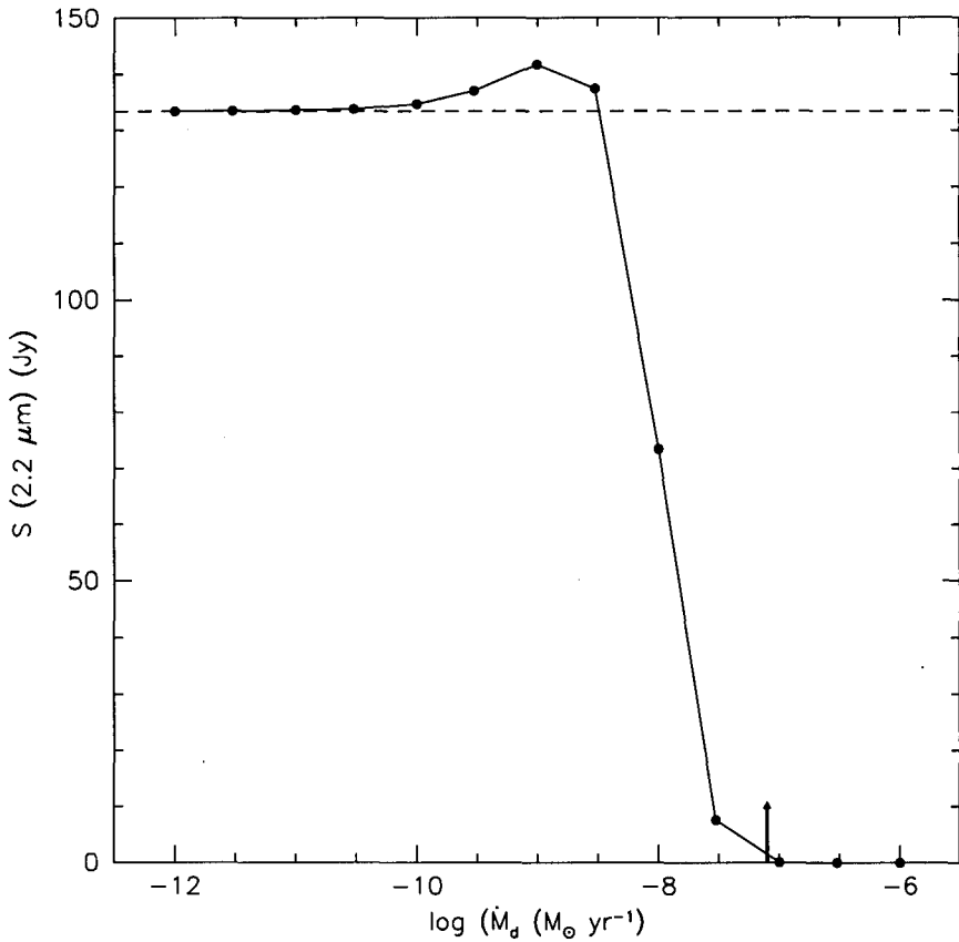
Figure 2. Emergent 2 \mu\text{m} flux density for an IRC+10216-like star ( L = 10^4 L_\odot , T_{\text{eff}} = 2500 \text{ K} ) at a distance of 1 kpc, versus dust ejection rate in M_\odot \text{ yr}^{-1} . The dashed line shows the photospheric flux density, and the heavy arrow indicates the approximate dust ejection rate for IRC+10216. The model assumes amorphous dust grains condensing at 1000 K above the photosphere, an outflow velocity of 14 km/sec, and a gas-to-dust ratio of 300 by mass.
