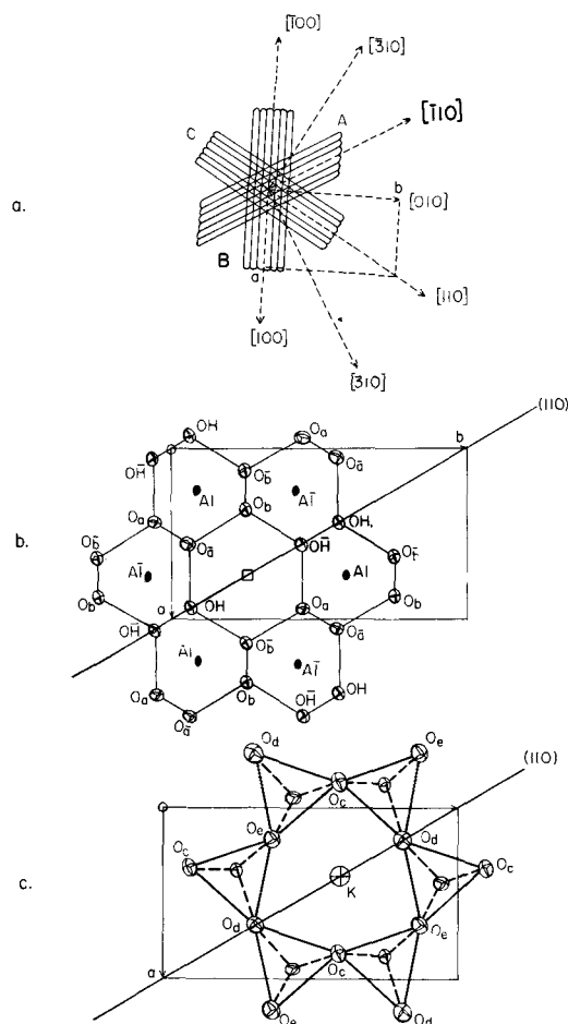
Fig. 2. (a) Orientation of illite aggregates consisting of lath-shaped crystallites with respect to the lattice directions of the 2M_1 unit cell. (b) The trace of the (110) plane, which is parallel to one set of lath-shaped crystallites in Fig. 2a, in the octahedral sheets of 2M_1 muscovite. This pseudo mirror plane passes through OHs and vacancies in octahedral sheets. (c) The trace of the (110) plane in the tetrahedral sheets passing through K and O d oxygens which are known to be tilted in 2M_1 dioctahedral micas.
