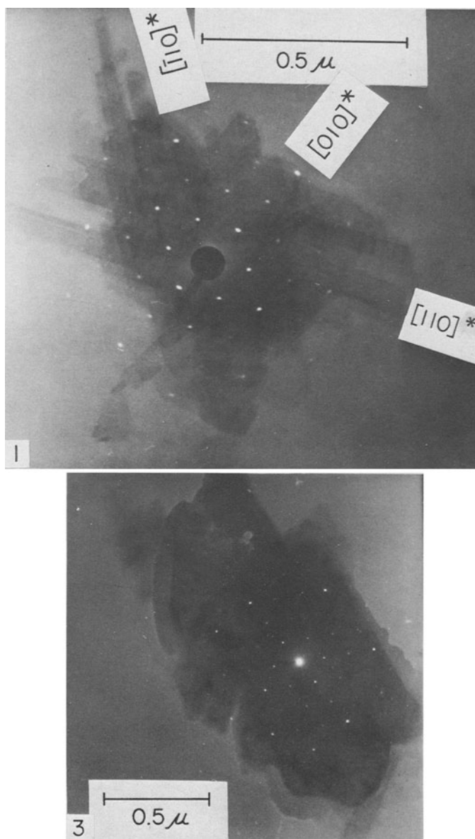
Fig. 1. Transmission electron bright field image of an illite aggregate from Marblehead. The SAD of the same aggregate is superimposed showing the strict orientational relationships of lath-shaped illite crystallites with respect to each other.
