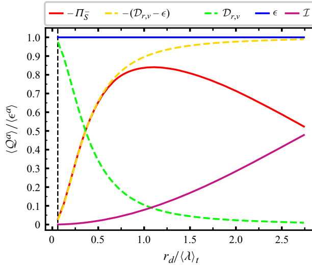
Figure 1. Non-zero spatiotemporal averages of surface-averaged terms of the solenoidal KHM equation (2.1) as functions of r_d / \langle \lambda \rangle_t . The vertical line marks the scale r_d = \langle \eta \rangle_t .
