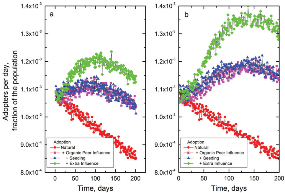
Fig. 7. Daily adoption curves for (a) persuasion ( \gamma = 0 ) and (b) susceptibility ( \gamma = 1 ). (color online)
