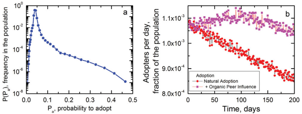
Fig. 2. (a) The distribution of spontaneous product adoption probabilities and (b) the simulated number of adopters per day under natural adoption and natural adoption + organic peer influence, \kappa = 0.5 . The plot represents persuasion-driven peer influence mechanism defined by \gamma = 0 . (color online)
