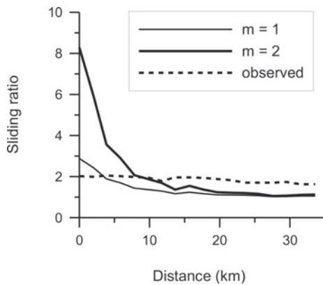
Fig. 7. Ratio of effective basal pressure in 1997 and 2005 for two values of the exponent m in the sliding relation (Equation (13)) and observed ratio of surface velocity in 2005 and 1995.
