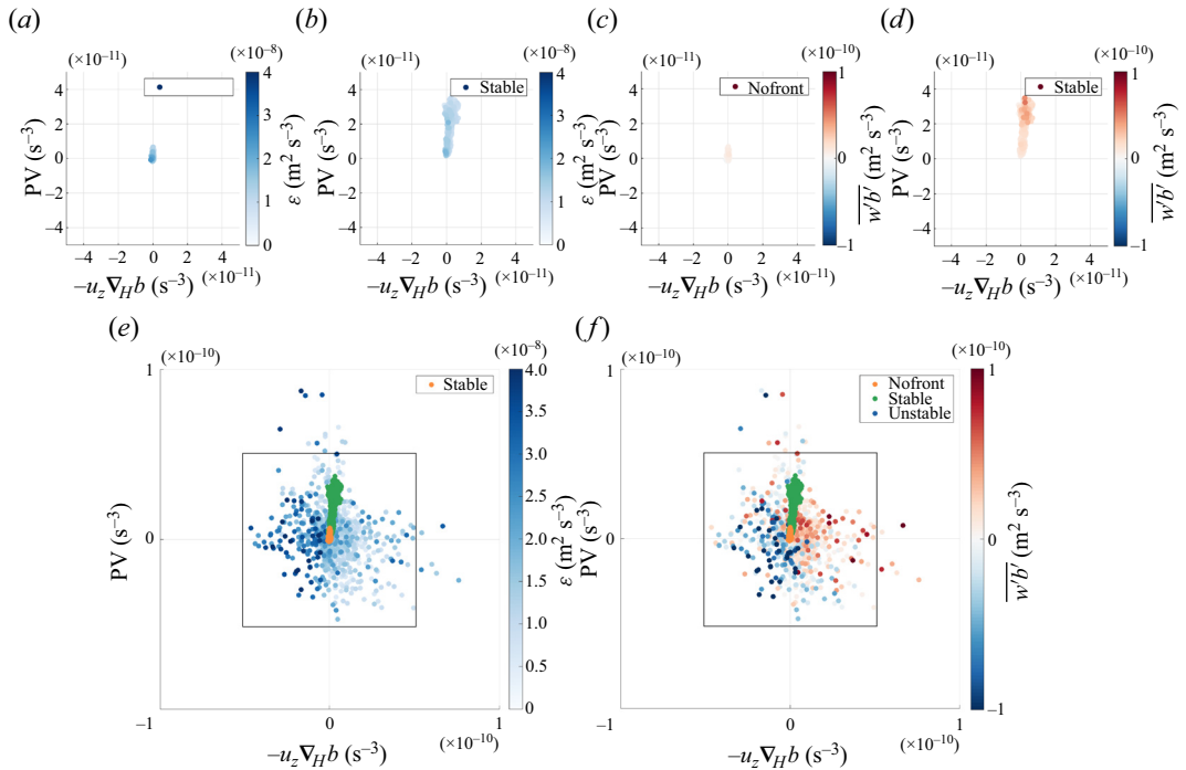
Figure 7. The correlation between PV (5.1) and the horizontal advection (ADV) of buoyancy by the horizontal shear, -\bar{u}_i/dz \bar{b}/dx_i (i.e. a horizontal advective term in the stratification tendency equation). The lower-left quadrant is destratifying flow with negative PV, and the upper-right quadrant is stratifying flow with positive PV. Dots are coloured by magnitude of \overline{w'b'} and \bar{\epsilon} : (a) NOFRONT \bar{\epsilon} , (b) STABLE \bar{\epsilon} , (c) UNSTABLE \bar{\epsilon} , and parameter space of STABLE and NOFRONT as in (a,b); (d) NOFRONT \overline{w'b'} , (e) STABLE \overline{w'b'} , (f) UNSTABLE \overline{w'b'} , and parameter space of STABLE and NOFRONT as in (d,e).
