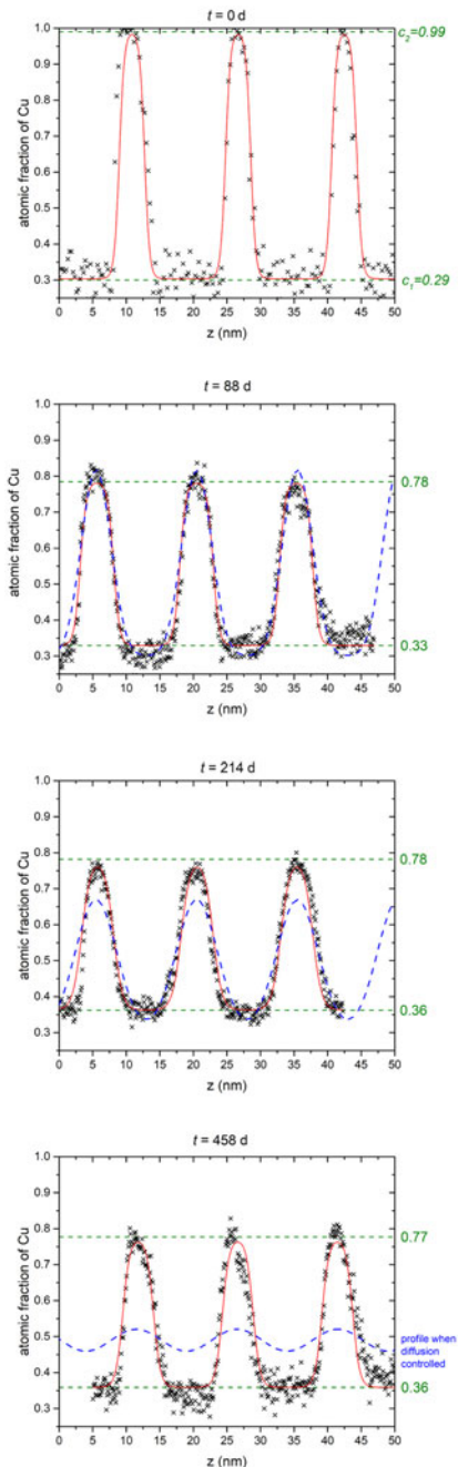
Fig. 7. Exemplary composition profiles for all annealing times of T = 573 K (black crosses) with the fit (red line) according to equation (4) and the plateau concentrations (green dashed line). The predicted profile is shown in the t = 458 d plot as a dashed blue line.
