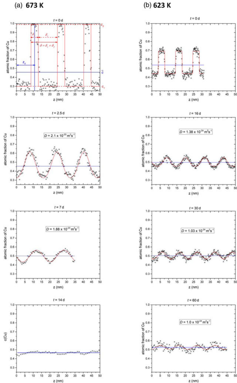
Fig. 5. Exemplary composition profiles for 673 K (a) and 623 K (b), black crosses) at different annealing times together with the fit (red line) according to equation (1) and the average concentration (blue line).
