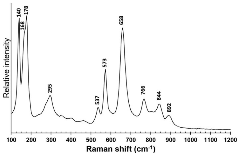
Fig. 2. Micro-Raman spectrum of bianchiniite in the range between 100 and 1200 \text{cm}^{-1} .
