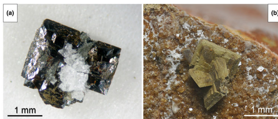
Fig. 1. (a) A loose aggregate of tabular crystals of bianchiniite, associated with 'hyalophane' and 'chlorite'. Holotype material was sampled from this specimen. (b) Deeply altered earthy tabular crystals of bianchiniite associated with rhombohedral crystals of siderite and whitish microcrystalline fibrous aragonite. Both specimens from the Sant'Olga level, Monte Arsiccio mine, Stazzema, Apuan Alps, Tuscany, Italy (in a private collection).
