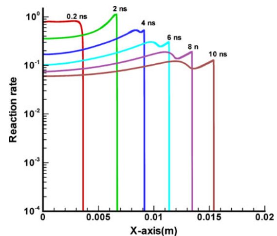
Fig. 8. Reaction rates (to be multiplied by 10^{36} \text{ m}^{-3}/\text{s} ) in solid DT at 1 ps pulse of energy flux E^* = 3 \times 10^8 \text{ J/cm}^2 KrF laser irradiation depending on the fuel depth x at different times up to 10 ns.
