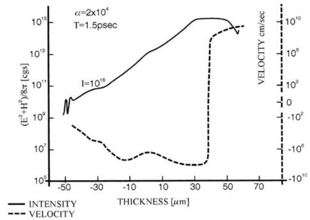
Fig. 2. 10^{18} W/cm 2 neodymium glass laser incident from the right-hand side on an initially 100 eV hot deuterium plasma whose density has a very low-reflecting bi-Rayleigh profile at initial time t = 1 , resulting in a laser energy density and a velocity distribution from plasma hydrodynamic computations at an interaction time t = 1.5 ps of interaction. The driving non-linear force is the negative of the varying energy density of the laser field (E^2 + H^2)/8\pi expressing the intensity. The dynamic development of temperature and density had accelerated the plasma block of about 20 vacuum wavelength thickness of the dielectric enlarged skin layer moving against the laser (positive velocity) and another block into the plasma (negative velocity) showing ultrahigh >10^{20} cm/s 2 acceleration.
