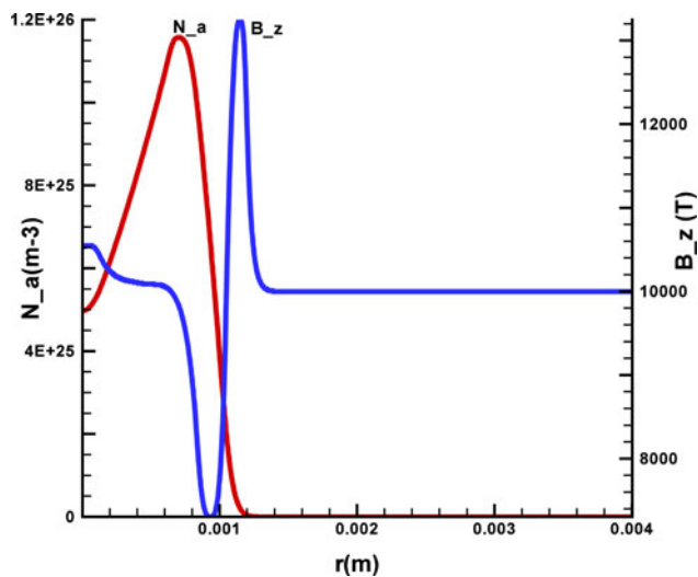
Fig. 13. Same case as Figure 11: Solid HB11 cylinder of 1 mm radius irradiated by ps- 10^{20} W/cm 2 laser pulse of 248 nm wavelength. Radial density at 100 ps of primary produced \alpha -particles N_a ending at 1 mm laser irradiation radius and the magnetic field strength depending on the radius r (in untouched fuel 10 kT at radius above 1 mm).
