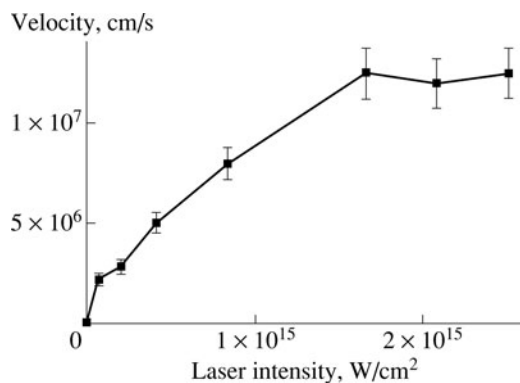
Fig. 4. Intensity dependence of the velocity of the plasma front from the Doppler line shift of the reflected from the irradiation of 700 fs KrF laser pulses on an aluminum target (Földes et al. , 2000).
