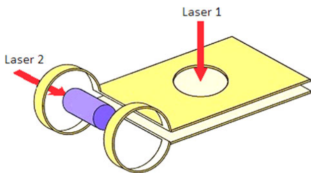
Fig. 10. Generation of a 5 kT magnetic field in the coils (Fujioka et al. , 2013) by firing a > \text{kJ} ns laser pulse 1 into the hole between the plates. The HB11 fusion fuel is coaxially located in the coils and the block ignition of the fusion flame is produced by the ps laser pulse for block ignition from laser 2.
