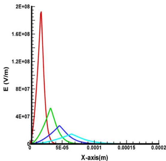
Fig. 7. Longitudinal electric field E as in case of Figure 1 for E^* = 10^8 \text{ J/cm}^2 depending of the depth X at times of 40 ps; 400 ps; 1 ns; 2 ns from the highest maximum, respectively.
