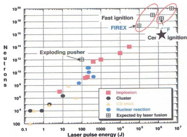
Fig. 1. Measured highest DT fusion neutron gains N per incident laser energy (full signs) of laser pulses in the range of ns duration (Hora, 2013a) with the highest value reported (Hurricane et al. , 2014) given by an asterisk.
