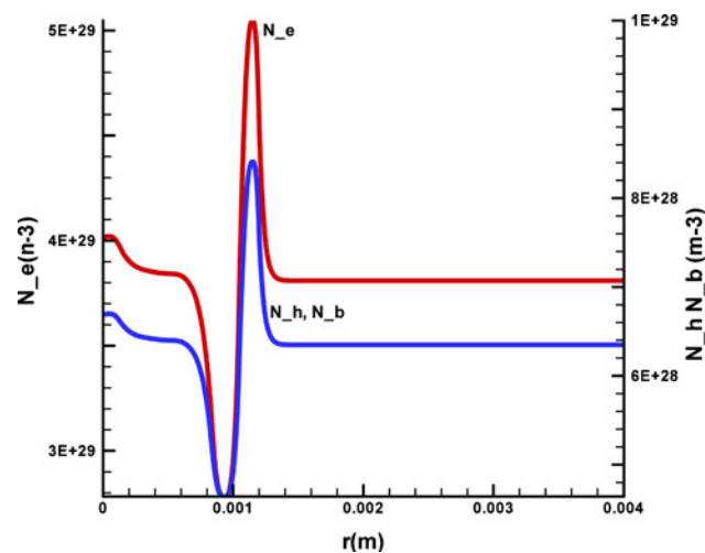
Fig. 11. Solid HB11 cylinder of 1 mm radius irradiated by a ps- 10^{20} \text{ W/cm}^2 laser pulse of 248 nm wavelength at concentric radius of 1 mm. After 100 ps, the dependence on the radius r is shown for the density of electrons N_e , boron N_b and hydrogen N_h (sequence at r = 0 from above) using a 10 kT magnetic field (Lalousis et al. , 2015).
