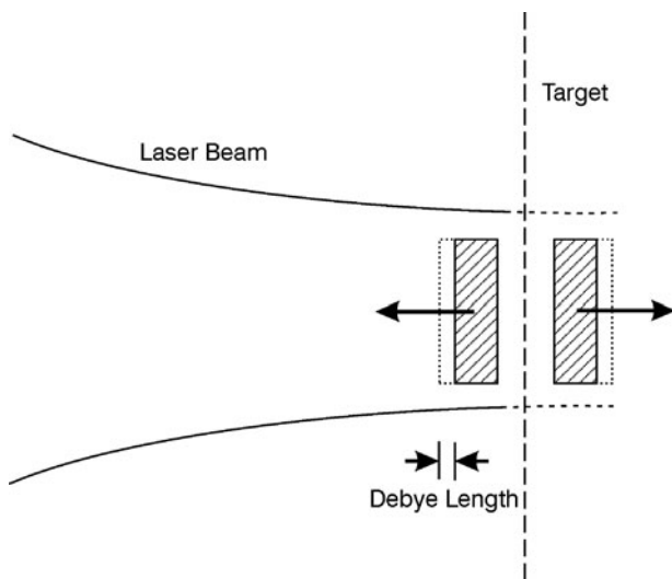
Fig. 3. Scheme of skin depth laser interaction, where the non-linear force accelerates a plasma block against the laser light and another block toward the target interior. In front of the blocks are electron clouds of the thickness of the effective Debye lengths [Eq. (5)] (Hora et al. , 2002b).
