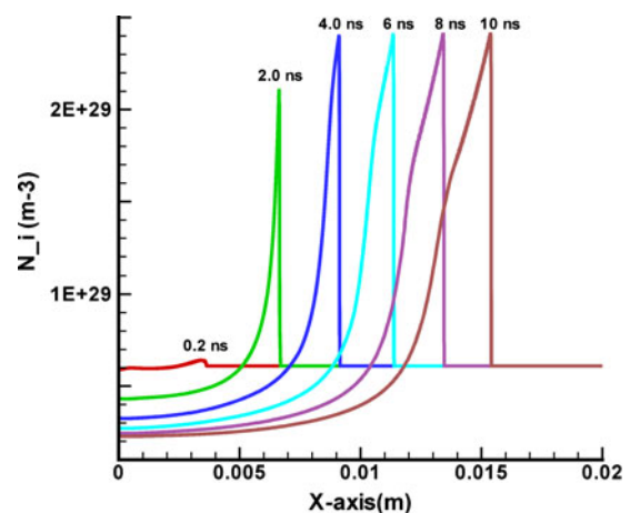
Fig. 5. Ion densities N_i depending of the depth X after a 1 ps 3 \times 10^8 J/cm 2 laser pulse of 248 nm wavelength has irradiated solid density DT. Parameter is the time after the ps interaction.
