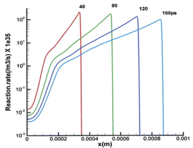
Fig. 14. HB11 fusion reaction rate at different depths x in 1D computation parallel to the magnetic field, at times after the ps generation of the fusion flame initiated by 10^{20} W/cm 2 , ps, 248 nm wavelength laser pulse.
