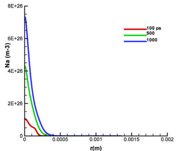
Fig. 15. \alpha density N_a depending on the radius r at different times (from lowest to highest curves for 100, 500 and 1000 ps, respectively) showing ignition from the increase of the curves on time (Lalousis et al. , 2014).
