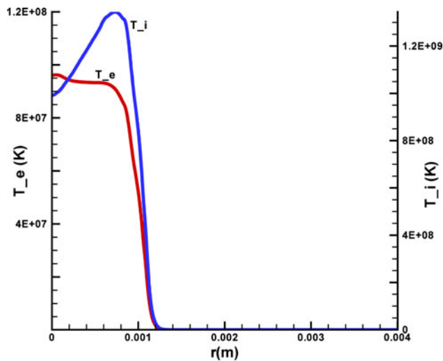
Fig. 12. Same as Figure 11 with electron and ion temperatures.
