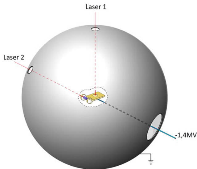
Fig. 16. The HB11 fusion without a radioactive radiation problem is based on a block ignition Hora et al. (2007) with a 30 kJ-ps laser pulse 2 (Fig. 10) where the solid hydrogen–boron fuel in the cylindrical axis of the magnetic coil is trapped by a 10 kT field sustained for about 1 ns after being generated by a laser pulse 1 of comparable duration. The central reaction unit (Fig. 10) is electric charged to the level of -1.4 million volts against the wall of a sphere producing \alpha -particles (He nuclei) of more than a GJ energy, of which a small part is needed for the operation of the laser pulses. One part of the gained costs of electricity is needed for the apparatus of the central reaction and for the boron metal of the fuel being destroyed at each reaction (Hora et al., 2014a).
