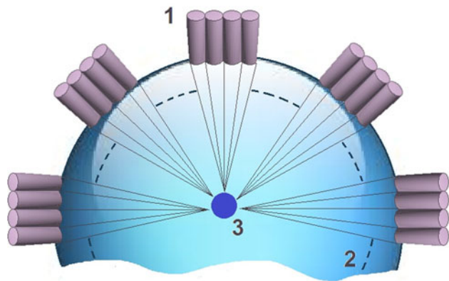
Fig. 9. Generation of a spherical shrinking laser pulse from radially directed fiber ends at a radius 1 to irradiate a spherical solid state fusion fuel 3 with the concentric grid 2 of positive electric charge for slowing down the generated \alpha -particles from the HB11 reactions (Hora et al. , 2014a).
