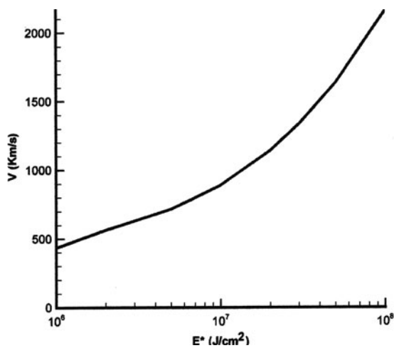
Fig. 6. Velocity V of the fusion flame at 2 ns after the initiating ps laser pulse of 248 nm wavelength depending on the energy flux E^* .
