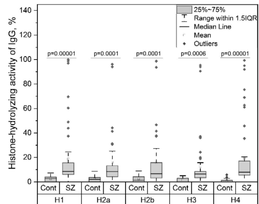
Fig. 1. Histone-hydrolyzing activity of IgG.
