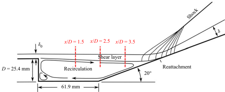
Figure 3. Cross-section of experimental configuration (from Baca 1982).
