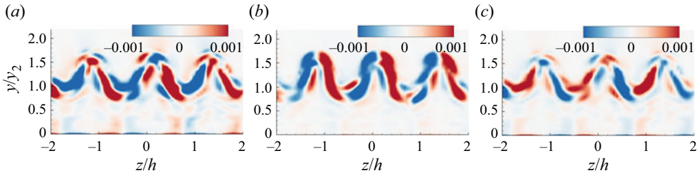
Figure 22. Time evolution of the conjugate modes 3 and 4; (a) t_0 , (b) t_0 + T/4 and (c) t_0 + T/2 .
