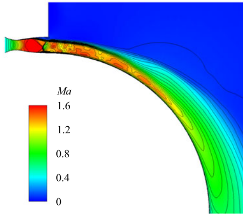
Figure 7. Effect of grid resolution on mean flow structure: coarse (colour contours), and fine grid (black lines).
