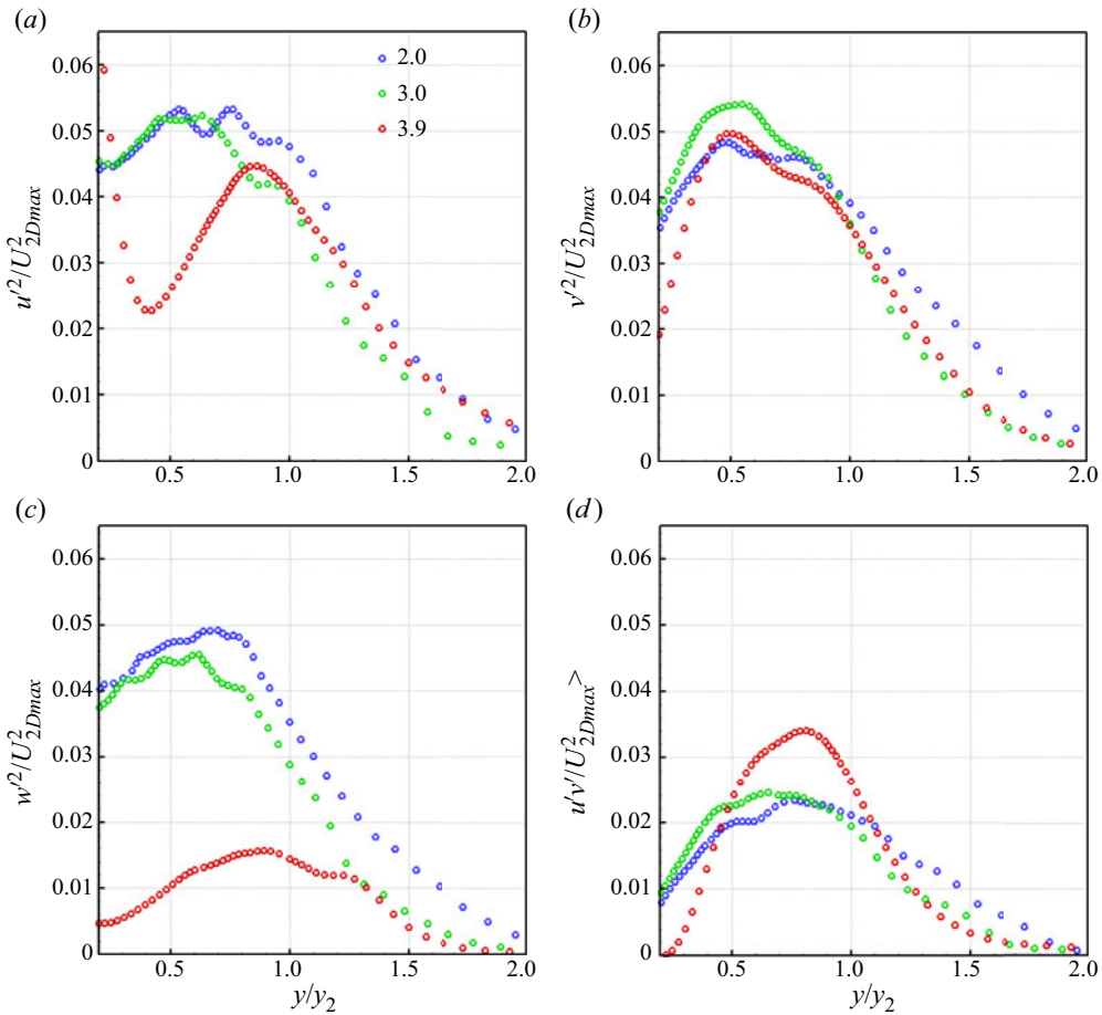
Figure 49. Reynolds stresses similarity profiles for all three M_c cases; (a) \overline{u'^2}/U_{2Dmax}^2 , (b) \overline{v'^2}/U_{2Dmax}^2 , (c) \overline{w'^2}/U_{2Dmax}^2 and (d) \overline{u'v'}/U_{2Dmax}^2 .
