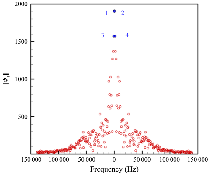
Figure 20. The DMD mode energy as the function of frequency.
