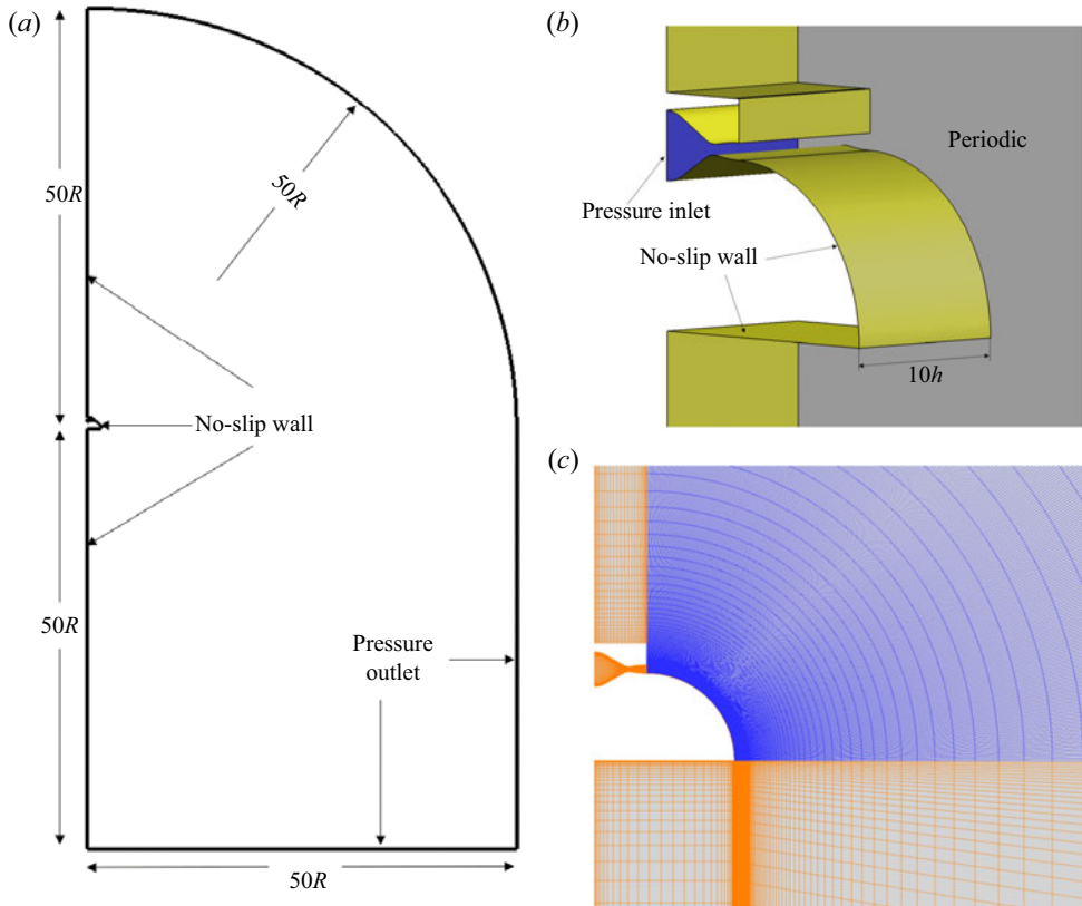
Figure 1. Schematics of (a), (b) computational domain and boundary conditions, and (c) grid around the curved wall.
