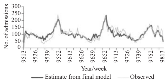
Fig. 3. Comparison of observed weekly number of unspecified pneumonia hospitalizations in children < 5 years of age with estimated weekly number due to RSV, influenza, and parainfluenza, S. pneumoniae , and M. pneumoniae based on the final model pneumonia shown in Table 6.
