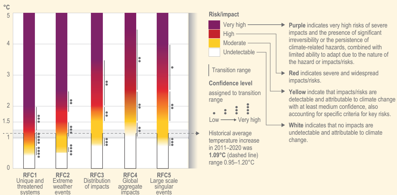
Figure FAQ16.5.1 | Simplified presentation of the five Reasons for Concern burning ember diagrams as assessed in this report (adapted from Figure 16.15).
