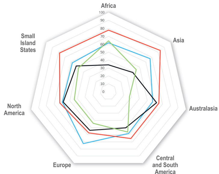
Figure 16.5 | Type of adaptation responses by global region. Percentages reflect the number of articles mentioning each type of adaptation over the total number of articles for that region. Radar values do not total 100% per region since publications frequently report multiple types of adaptation; for example, construction of drainage systems (infrastructural), changing food storage practices by households (behavioural), and planting of tree cover in flood-prone areas (nature-based) in response to flood risk to agricultural crops. Data updated and adapted from Berrang-Ford et al. (2021a), based on 1682 scientific publications reporting on adaptation-related responses in human systems.
