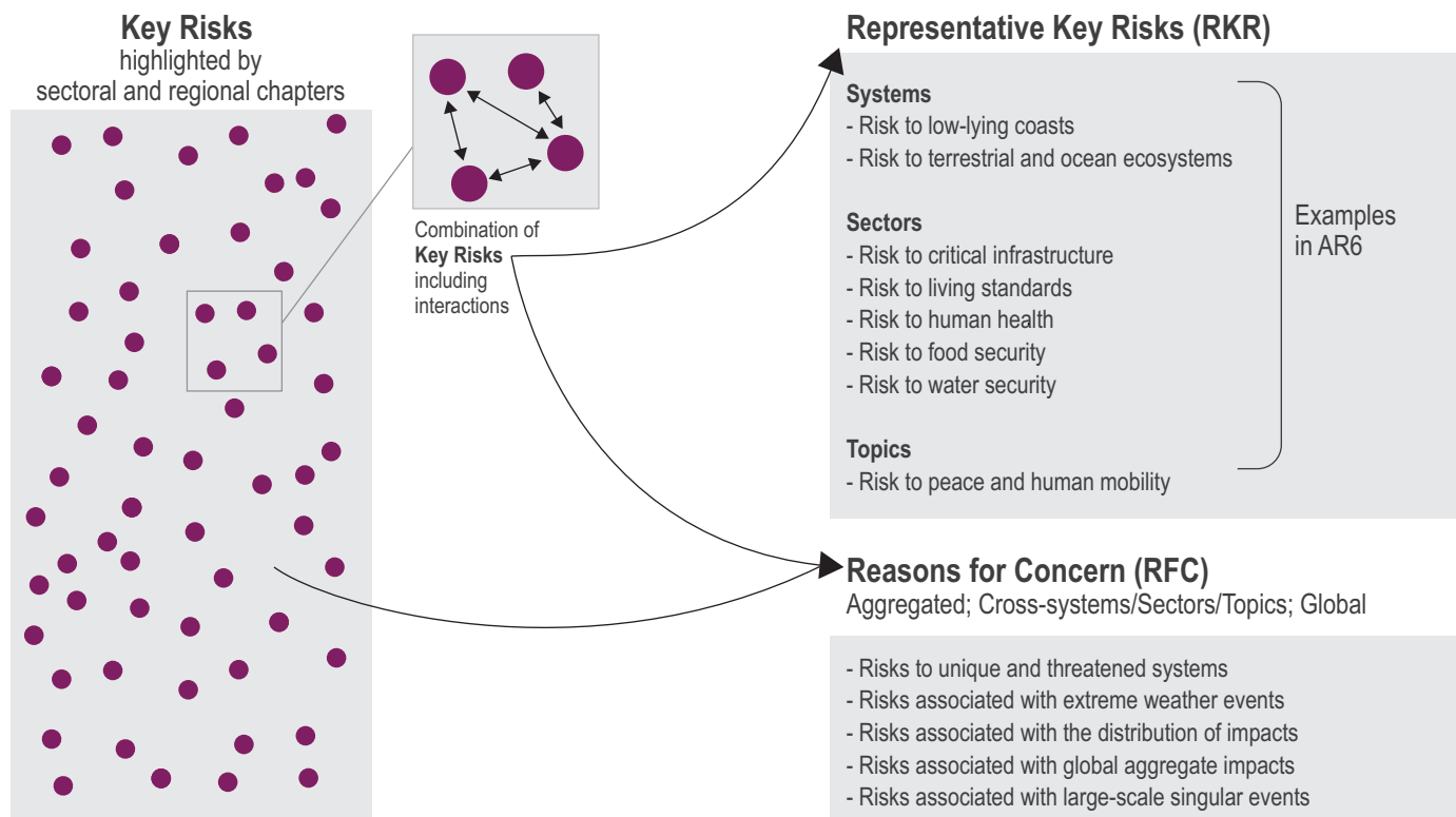
Figure 16.13 | Interconnections between the key risks, representative key risks and Reasons for Concern.
