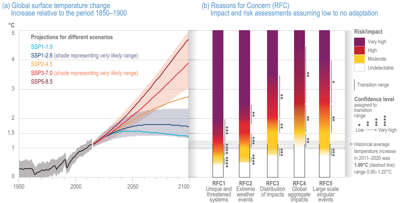
Figure 16.15 | The dependence of risk associated with the Reasons for Concern (RFCs) on the level of climate change, updated by expert elicitation and reflecting new literature and scientific evidence since AR5 and SR15.
