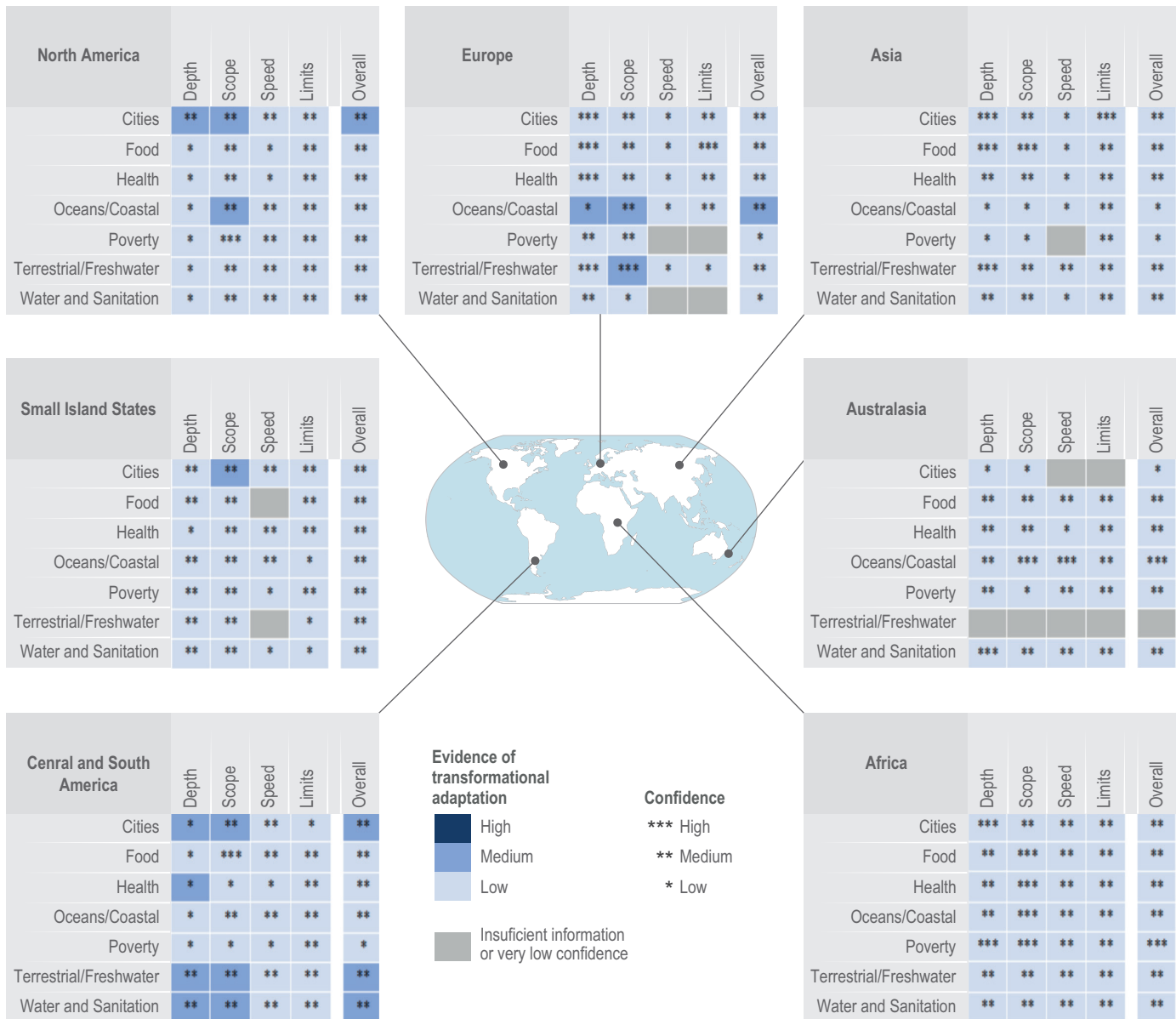
Figure 16.6 | Evidence of transformative adaptation by sector and region. Evidence of transformational adaptation does not imply effectiveness, equity or adequacy. Evidence of transformative adaptation is assessed based on the scope, speed, depth and ability to challenge limits of responses reported in the scientific literature (see Supplementary Material for methods). Studies relevant to multiple regions or sectors are included in assessment for each relevant sector/region.
