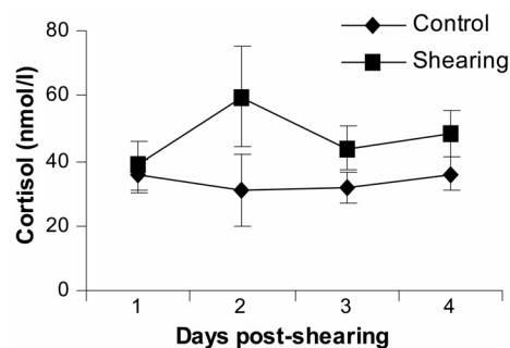
Figure 3 Cortisol response to shearing in captive vicunas.
