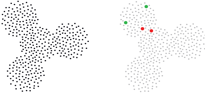
FIGURE 1.1. Four clusters?
