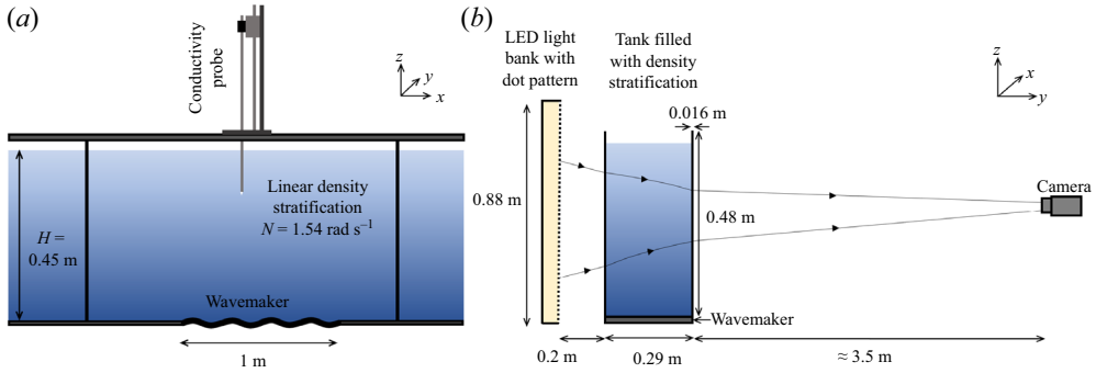
Figure 1. (a) A schematic showing the front view of the tank as would be seen by the camera. The wavemaker is located along a 1 m section of the tank floor, 2.5 m and 7.5 m away from the left and right boundary wall, respectively. The tank is filled with a 0.45 m salt stratification. A conductivity probe, mounted above the tank, measures the density profile. (b) A schematic showing the side view of the tank in order to visualise the optical arrangement for synthetic schlieren. The thermal tunnel is not shown for clarity.
