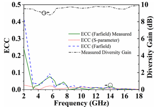
Figure 13. Measured ECC and DG of the recommended antenna.
