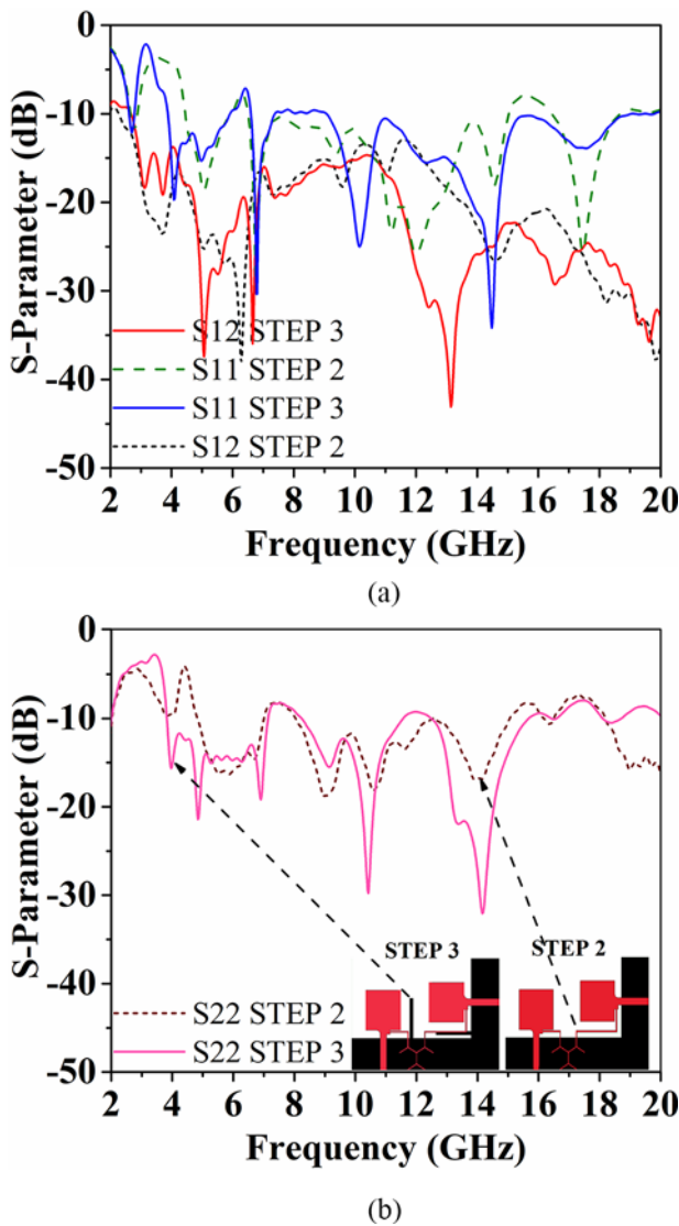
Figure 5. Scattering parameters of the radiator in the presence and absence of the extended ground stubs. (a) Comparison among S11 and S12 for STEP 2 and 3 and (b) comparison among S22 for STEP 2 and STEP 3.
