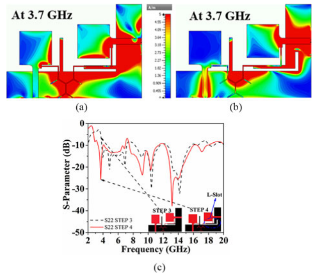
Figure 6. The surface current spread over the radiator at (a) 3.7 GHz without the L -shaped slot, (b) 3.7 GHz with the L -shaped slot, and (c) comparison of S_{22} with and without the L -slot up on the ground structure.
