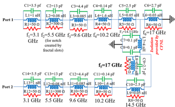
Figure 10. Equivalent circuit of the proposed antenna.
