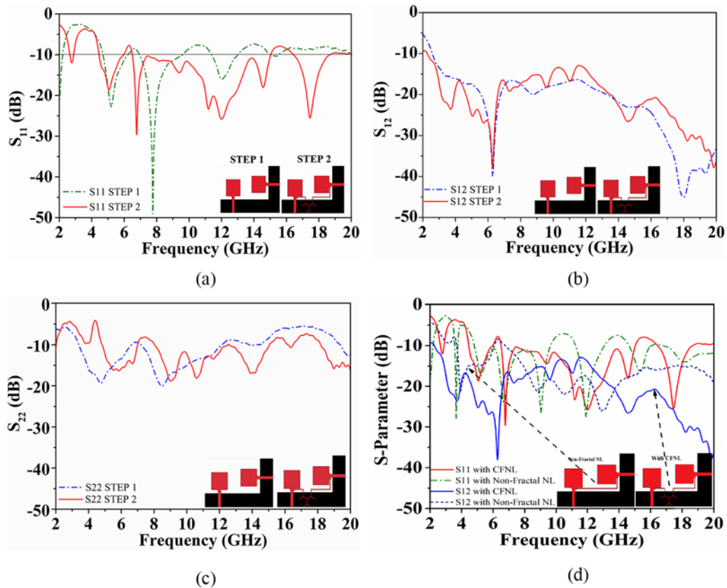
Figure 2. Analysis of S-parameter with an application of CFNL. (a) Comparison of S11, (b) S12, and (c) S22 after the application of CFNL and (d) comparison between application of fractal and non-fractal NL for impedance matching and isolation improvement.
