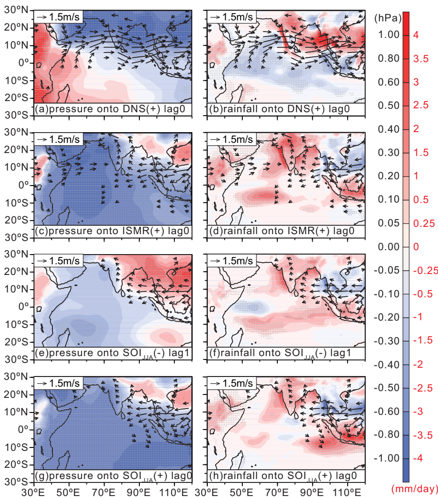
Figure 2. (Colour online) (a) Regression coefficients of JJAS surface pressure (shaded) and 850 hPa horizontal winds (vector) against the normalized time series of ISMR wind index (DNS). (b) is the same as (a) but with surface pressure replaced by JJAS rainfall (shaded). (c)–(d), (e)–(f), (g)–(h) are the same as (a)–(b) but for regression coefficients against the normalized time series of ISMR, of SOI_{JJA}*(-1) in 1 year before, and of SOI_{JJA} in the same year, respectively. Unless otherwise stated, grey dotted areas in all regression figures are significant at the 95% level with Student's t -test, and small wind vectors (magnitude < 0.5 m/s) are not shown for clarity. For regression results, the character “(+)” or “(-)” means the normalized time series was multiplied by +1 or -1, and the character “lag0” or “lag1” means dependent variable lags independent variable (or the normalized time series) by 0 or 1 year.
