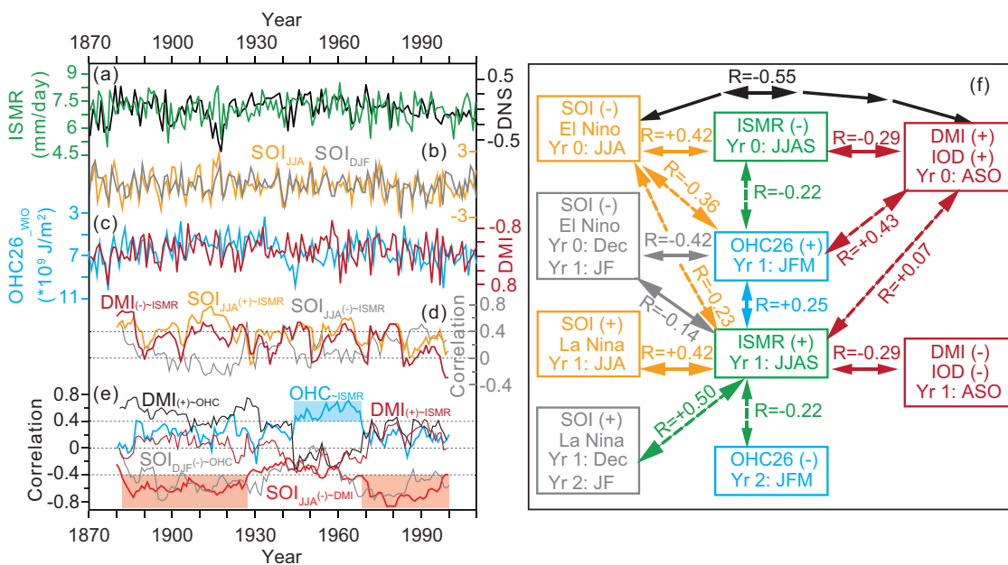
Figure 1. (Colour online) (a) Modern observed time series of ISMR rainfall index (ISMR, green line) and ISMR wind index (DNS, with linear trend removed, no units) from the year 1871 to 2010 AD. (b) Time series of SOI indexes during DJF and JJA (gray line for SOI_{DJF} and orange line for SOI_{JJA} , no units). (c) ASO DMI index (brown line, units: K) is compared with the OHC26 WIO time series (cyan line). (d) 20-year moving correlations for ISMR in Yr 1 with three indexes: DMI(-) in Yr 1 (multiplied by -1, brown line), SOI_{JJA}(+) in Yr 1 (orange line), SOI_{JJA}(-) in Yr 0 (gray line). (e) Moving correlations for OHC26 WIO in Yr 1 with three indexes: ISMR(+) in Yr 1 (cyan line), DMI(+) in Yr 0 (black line), SOI_{DJF}(-) in Yr 1 (gray line), and for DMI(+) in Yr 0 with two indexes: ISMR(+) in Yr 1 (brown line), SOI_{JJA}(-) in Yr 0 (red line). (f) Lead-lag correlations (R) between different time series. In (d), (e), and (f), those positive or negative signs in parentheses show the anomalous status of SOI, DMI, OHC26, and ISMR in the corresponding year.
