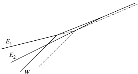
FIGURE A3. \mathfrak{d} \rightarrow \mathfrak{d}^- (second curve).
