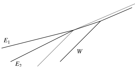
FIGURE A4. \mathfrak{d} \rightarrow \mathfrak{d}^+ .
