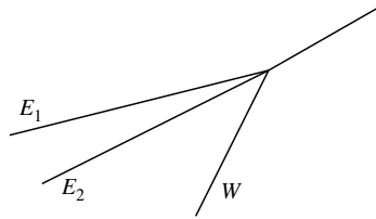
FIGURE A5. A codimension 1 singularity, second case.
