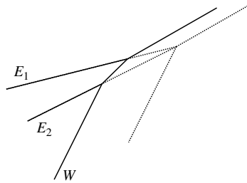
FIGURE A6. \mathfrak{d} \rightarrow \mathfrak{d}^- .
