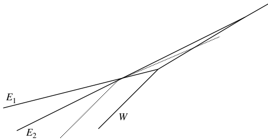
FIGURE A8. \mathfrak{d} \rightarrow \mathfrak{d}^+ (second curve).
