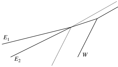
FIGURE A7. \mathfrak{d} \rightarrow \mathfrak{d}^+ (first curve).
