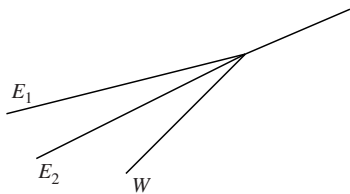
FIGURE A1. A codimension 1 singularity, first case.
