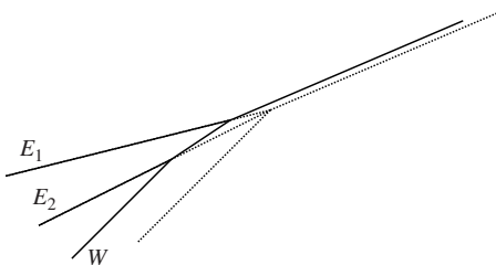
FIGURE A2. \mathfrak{d} \rightarrow \mathfrak{d}^- (first curve).
