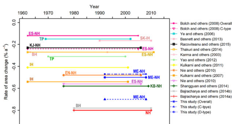
Fig. 10. Rates of area change from different studies for glaciers around the Himalayas: Everest South (ES), Tibetan Plateau (TP), Sikkim (SK), Kanchenjunga (KJ), Bhutan Himalaya (BH), Indian Himalaya (IH), Nepal Himalaya (NH), Everest North (EN) and Koshi Basin (KB).
