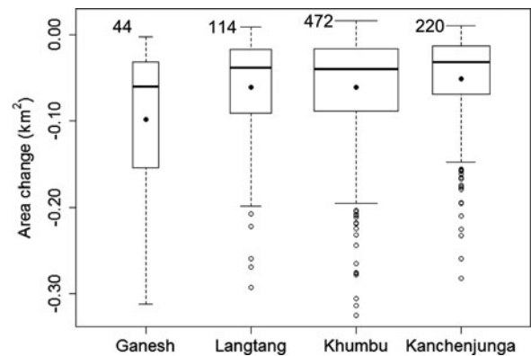
Fig. 11. Glacier area change for the four massifs studied in the eastern Nepal Himalaya. The box width denotes the glacier number. The upper and lower bounds of the box, thick lines and solid circles denote the first and third quartiles, median and average of the area change, respectively. The whiskers extend 1.5 times the interquartile range from the box. Outliers beyond -0.40 km 2 (one in Ganesh, four in Khumbu and one in Kanchenjunga) are not shown.
