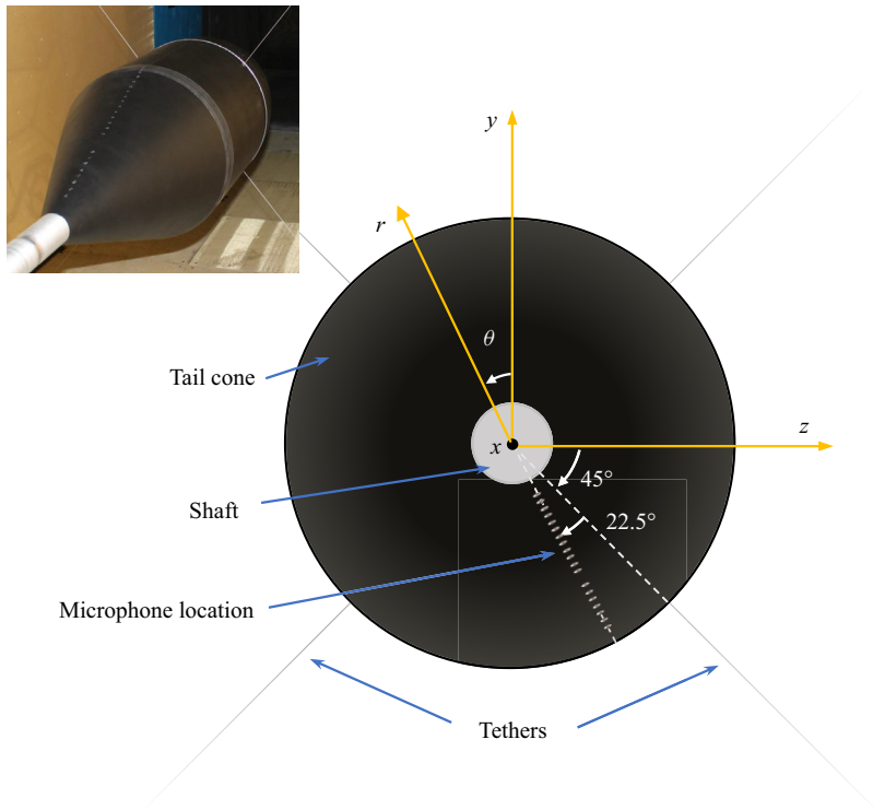
Figure 2. Schematic showing the circumferential location of the surface microphones on the tail cone with respect to the tethers. The view corresponds to that seen by an observer located downstream of the BOR and viewing directly upstream.
