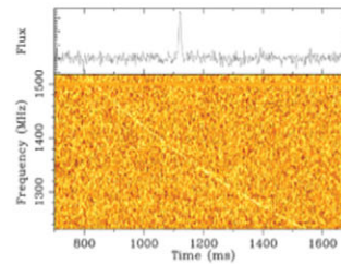
Frequency vs time waterfall plot for FRB010125. Not bandpass corrected.
