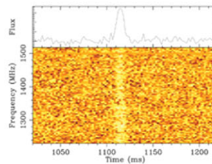
Frequency vs. time waterfall plot for FRB010125 dedispersed to the optimal DM. Not bandpass corrected.
