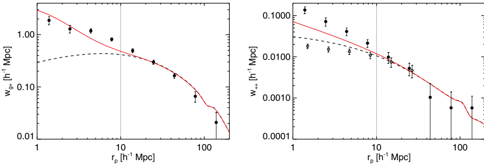
Figure 1. The projected correlation function between galaxy position and shape w_{g+} (left panel) and projected shape autocorrelation w_{++} (right panel) are shown as a function of projected separation, r_p . Data points show the measurements of Okumura et al. 2009, Okumura & Jing 2009. The w_{++} measurements have been projected along the line-of-sight, and open circles indicate the original measurement without a correction required to account for source clustering - see Blazek et al. 2011 for more information. Dashed lines indicate the linear order prediction of the tidal alignment model, while solid lines include the Halofit correction for nonlinear dark matter clustering (Smith et al. 2003).
