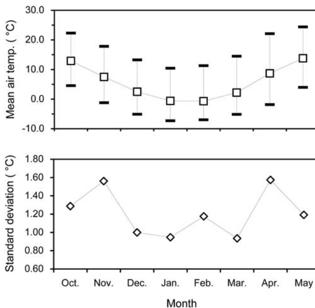
Fig. 4. Fluctuations in the mean air temperature and its standard deviation during the winter season. The error bars show the maximum and minimum mean temperatures recorded over the 11 years.
