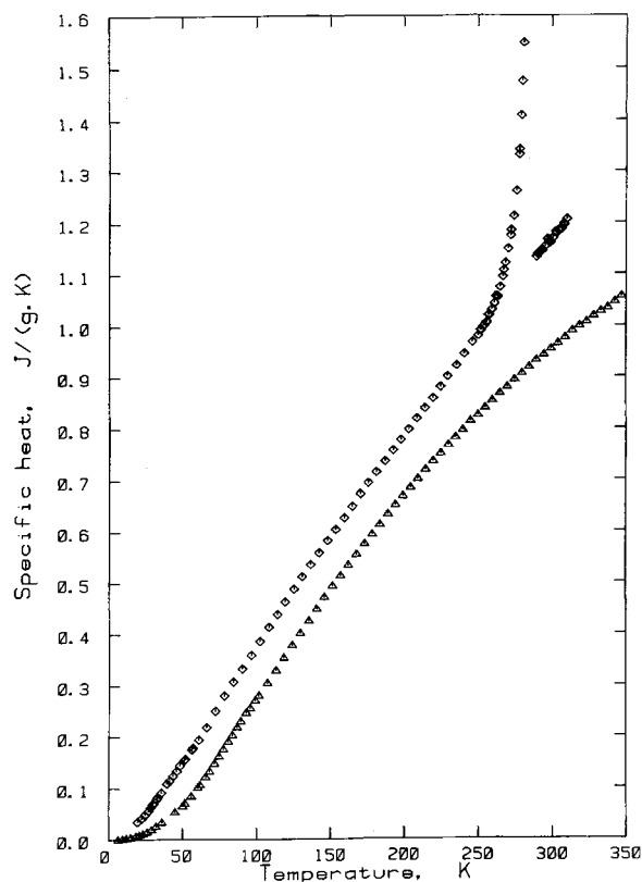
Figure 2. Specific heats of kaolinite (triangles) and kaolinite:DMSO intercalate (diamonds) measured by adiabatic calorimetry.
