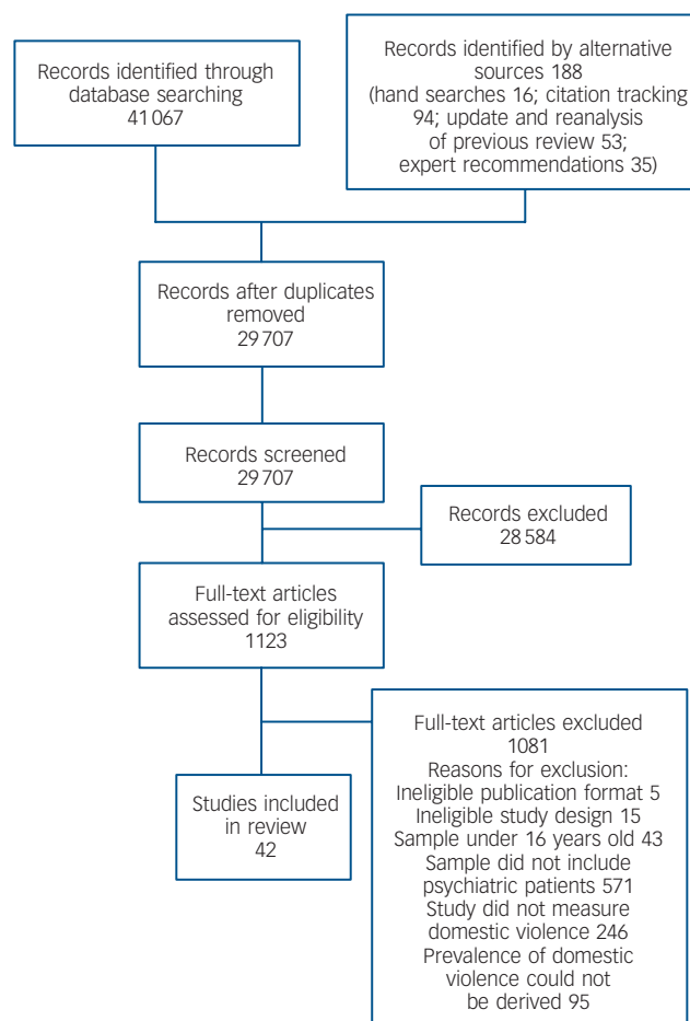
Fig. 1 Study selection.
