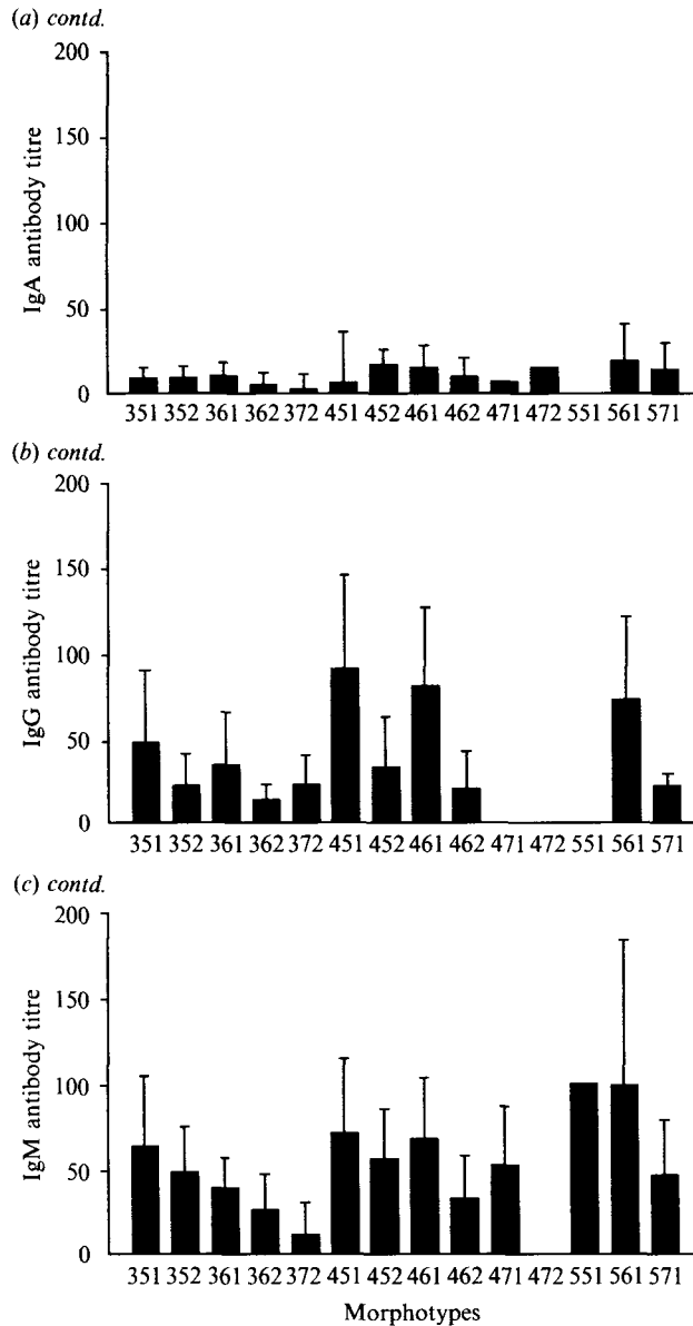
Fig. 2(a) Mean ( \pm s.d.) plasma antibody titres of the IgA isotype against objects composing the faecal flora of ten healthy individuals. (b) Mean ( \pm s.d.) plasma antibody titres of the IgG isotype against objects composing the faecal flora of ten healthy individuals. (c) Mean ( \pm s.d.) plasma antibody titres of the IgM isotype against objects composing the faecal flora of ten healthy individuals.
