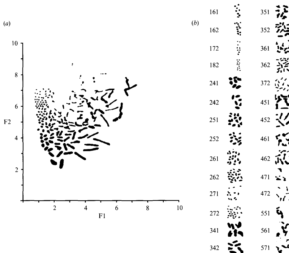
Fig. 1(a) Faecal objects (mainly bacteria) of a healthy volunteer are depicted according to their scores of the morphological parameters F1 and F2. The axes were divided in ten equal parts, according to which the morphotypes were defined. (b) Representative forms of objects belonging to the 28 morphotypes.
