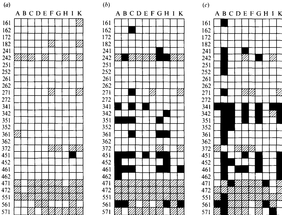
Fig. 3 (a) The IgA plasma antibody responses against his/her own faecal morphotypes are shown for each person (A–K). Titres higher than 64 are represented by black boxes whereas morphotypes with titres lower than 64 are left open (white boxes). When too few bacteria were found in a morphotype to calculate the titre, the box was hatched. (b) The IgG plasma antibody responses against his/her own faecal morphotypes are shown for each person (A–K). (c) The IgM plasma antibody responses against his/her own faecal morphotypes are shown for each person (A–K).
