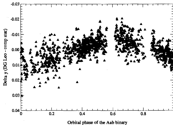
Fig. 1. Residual data of DG Leo phased with twice the orbital frequency.
