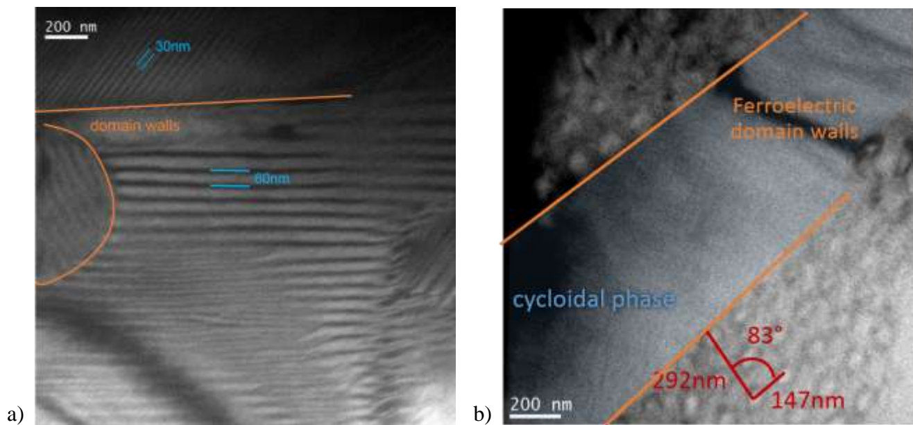
Figure 1. a) Cycloidal phase of GaV 4 Se 8 cut in <111> direction at 10K and 160mT: different sizes of the cycloidal phase are clearly visible; b) ferroelectric domains in GaV 4 Se 8 cut in <110> direction: ferroelectric domain walls separate cycloidal and skyrmion phase from each other
