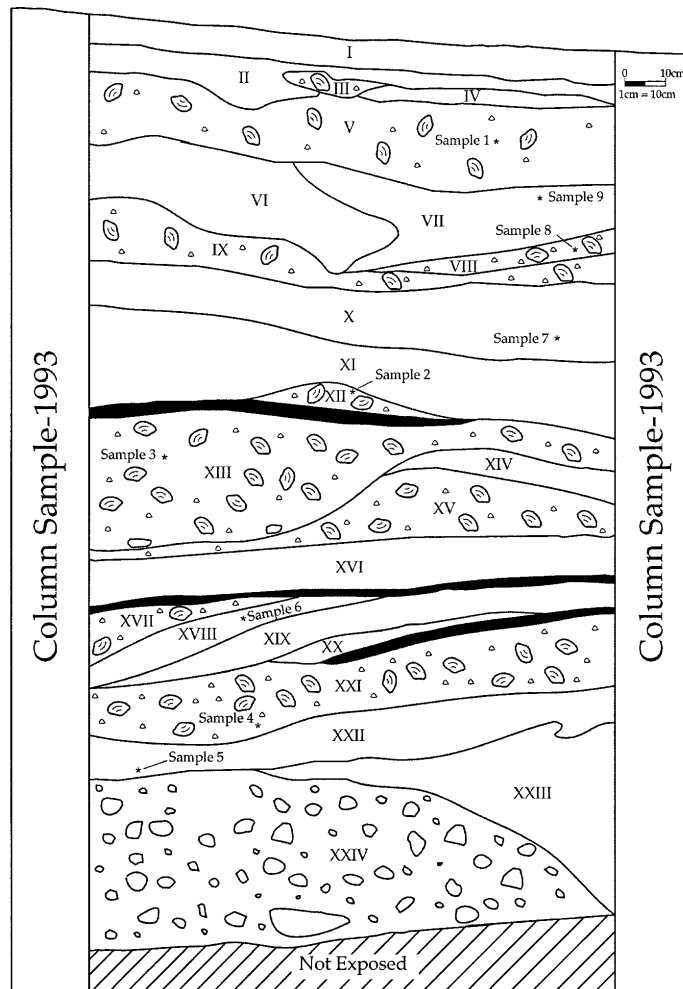
Figure 1 Stratigraphic section (railroad profile) indicating the position of shell and charcoal specimens that were collected for radiocarbon work
