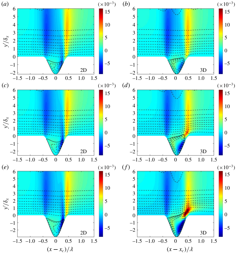
FIGURE 5. (Colour online) Comparison of 2-D base flows (a,c,e) and 3-D base flows in the planes z' = 0 (b,d,f). (a,b) h = 1.620 mm; (c,d) h = 1.895 mm; (e,f) h = 2.170 mm. The solid dark lines indicate the closed curves defined by \Gamma = \{(x', y') : \bar{u}'(x', y', z' = 0) = 0\} . The parameter \lambda is fixed and equals 40.5 mm. \bar{u}' (iso-lines) and \bar{v}' (coloured contours) are normalised by the free-stream velocity magnitude. (See table 1 for the parameters of Cases A–C of Group 2).
