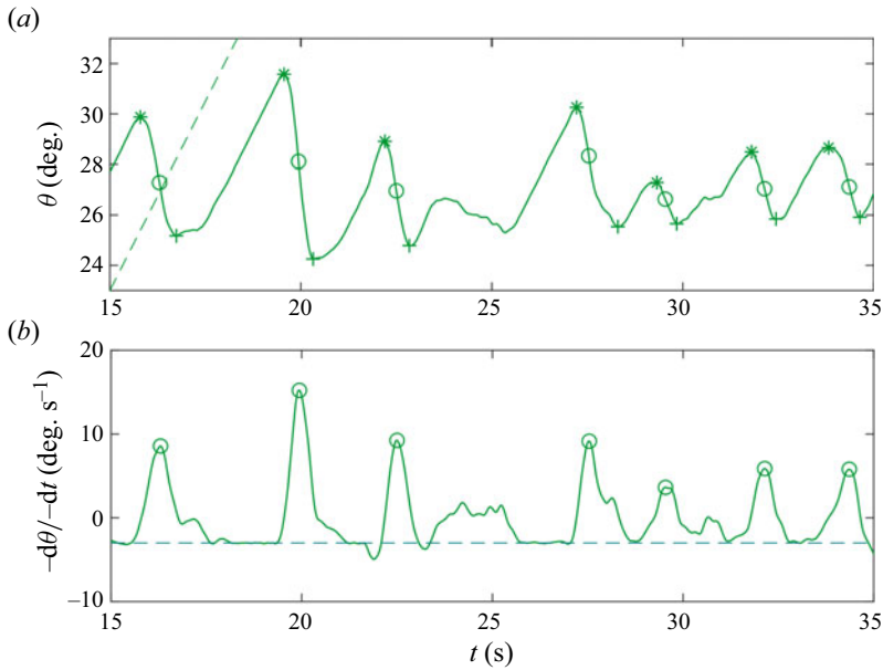
Figure 7. Processing of surface inclination history recorded in an experiment or discrete element simulation (here, a simulation by Kasper et al. 2021): (a) segmentation of angle history into separate avalanche events; (b) identification of extremal slope relaxation rates from numerically differentiated signal. Symbols: failure (stars), arrest (plus) and extremal values (circles). Dashes: drum rotation rate.
