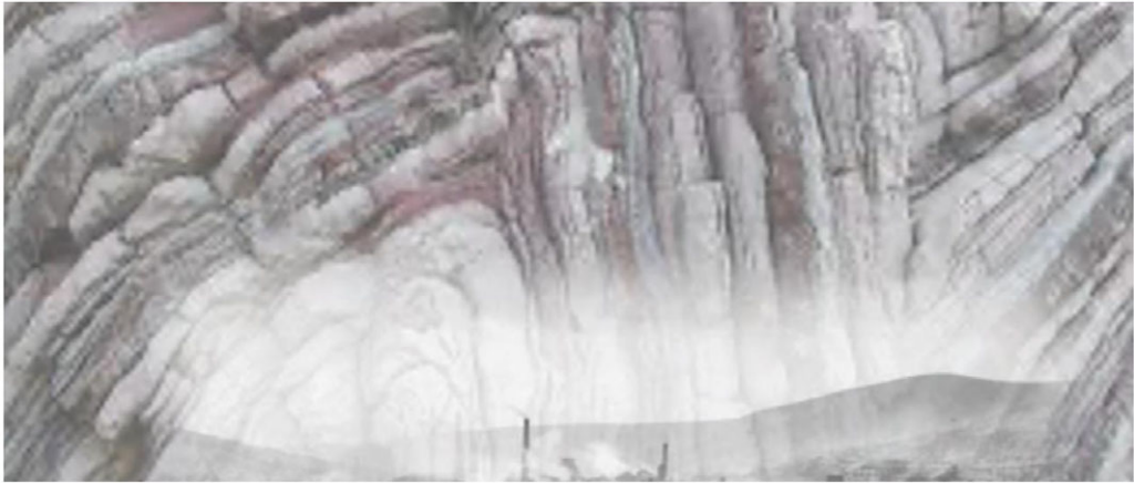
Figure 1. Syncline folds artist's impression.
