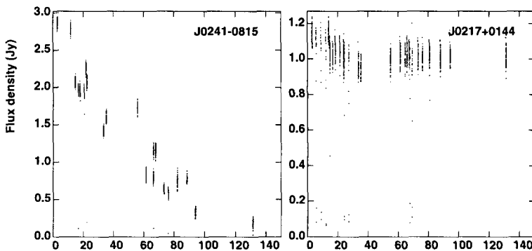
Figure 1. Flux density versus (u, v) distance in M\lambda for two representative sources.
