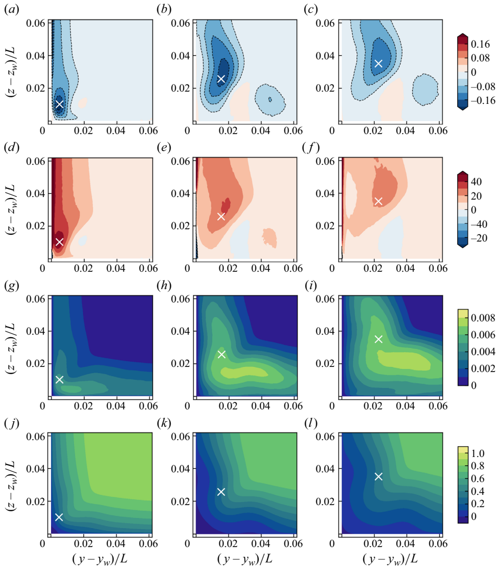
Figure 10. Production of the Reynolds shear stress \overline{u'v'} and its component near the corner at (a,d,g,j) x/L = 1.3 , (b,e,h,k) x/L = 1.4 and (c,f,i,l) x/L = 1.5 . The white cross symbols denote the location of the minimum Reynolds shear stress. Plots are for (a-c) -\overline{v'v'}(\partial\bar{u}/\partial y)/(u_\infty^3/L) , (d-f) \partial\bar{u}/\partial y/(u_\infty/L) , (g-i) \overline{v'v'}/(u_\infty^2) and (j-l) \bar{u}/u_\infty (reference).
