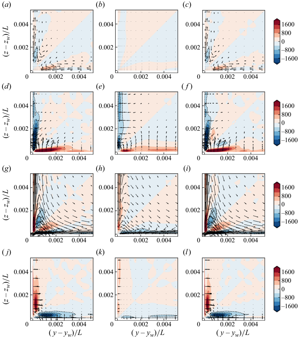
Figure 11. Streamwise vorticity budget near the corner at (a,d,g,j) x/L = 1.0 , (b,e,h,k) x/L = 1.5 and (c,f,i,l) x/L = 2.0 . Each term is normalized by u_{\infty}^2/L^2 . The in-plane fluxes (3.8) are overlaid as vectors; S_{\omega} and residuals are omitted because they are almost zero all over the cross-sections. Plots are for (a–c) C_{\omega} with vectors (C_{\omega,y}, C_{\omega,z}) , (d–f) R_{\omega} with vectors (R_{\omega,y}, R_{\omega,z}) , (g–i) A_{\omega} with vectors (A_{\omega,y}, A_{\omega,z}) and (j–l) V_{\omega} with vectors (V_{\omega,y}, V_{\omega,z}) .
