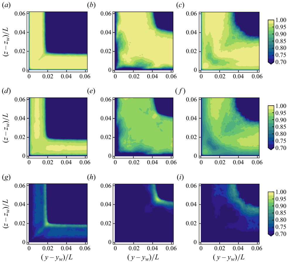
Figure 13. Tensorial inner product \sigma_{RS} distributions near the corner at (a,d,g) x/L = 1.0 , (b,e,h) x/L = 1.5 and (c,f,i) x/L = 2.0 , with different parameter values in (4.5): (a-c) proposed, (C_{q1}, C_{q2}) = (1.0, 0.5) ; (d-f) QCR2000 (Spalart 2000), (C_{q1}, C_{q2}) = (0.6, 0.0) ; (g-i) LCR, (C_{q1}, C_{q2}) = (0.0, 0.0) .
