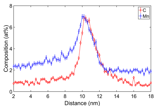
Fig. 2. Carbon and manganese composition profiles, red and blue, respectively, along a cylinder encompassing the entire interface within the dataset positioned perpendicular to the interface and with a step size of 0.2 nm.
