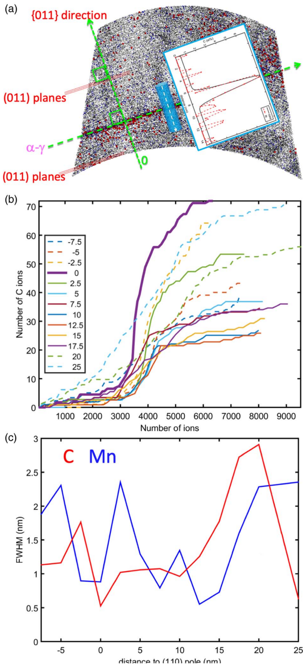
Fig. 3. (a) A 5-nm-thick slice through the data that show the interface edge-on and contain the trace of the two (011) poles and corresponding sets of (011) planes. Two normal axes are defined at the crossing between the interface and the poles. A succession of profiles is calculated within a 4-nm-diameter cylinder, and each profile is fitted with a Gaussian function, as shown in inset. (b) Integral profile for each of the corresponding profiles, the color reported in the legend indicates the distance to the pole. (c) FWHM of the fitted Gaussian function for the C (red) and Mn (blue).
