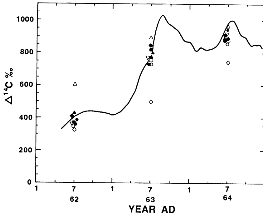
Fig. 2. Atmospheric ^{14}\text{CO}_2 concentrations as measured at Nordkapp ( 71^{\circ}06'\text{N} , 23^{\circ}59'\text{E} ) and Trondheim ( 63^{\circ}\text{N} , 10^{\circ}\text{E} ) (Nydal & Lövseth 1983) and ^{14}\text{C} concentration in organic samples from various latitudes. \Delta = Mackenzie delta ( 68^{\circ}\text{N} , 130^{\circ}\text{E} ) (Dai & Fan 1986); \square = Lowland USSR ( 60^{\circ}\text{N} , 31^{\circ}\text{E} ) (Kolesnikov, Gorshkova & Biryulin 1970); \diamond = Mingyin, China ( 27^{\circ}\text{N} , 100^{\circ}\text{E} ) (Dai & Fan 1986); \blacktriangle = Treeless Height, USSR (Kolesnikov, Gorshkova & Biryulin 1970); * = Copenhagen, Denmark ( 56^{\circ}\text{N} , 13^{\circ}\text{E} ) (Tauber 1967); \blacklozenge = Kiel, Germany ( 54^{\circ}\text{N} , 10^{\circ}\text{E} ) (Willkomm & Erlenkeuser 1968); \circ = Quillayute, USA ( 48^{\circ}\text{N} , 125^{\circ}\text{W} ) (Grootes et al. 1989); \nabla = Dailing, China ( 48^{\circ}\text{N} , 129^{\circ}\text{E} ) (Dai & Fan 1986); \bullet = New York, USA ( 41^{\circ}\text{N} , 74^{\circ}\text{W} ) (Cain & Suess 1976); \blacksquare = Georgia, USSR ( 38^{\circ}\text{N} , 45^{\circ}\text{E} ) (Burchuladze et al. 1989).
