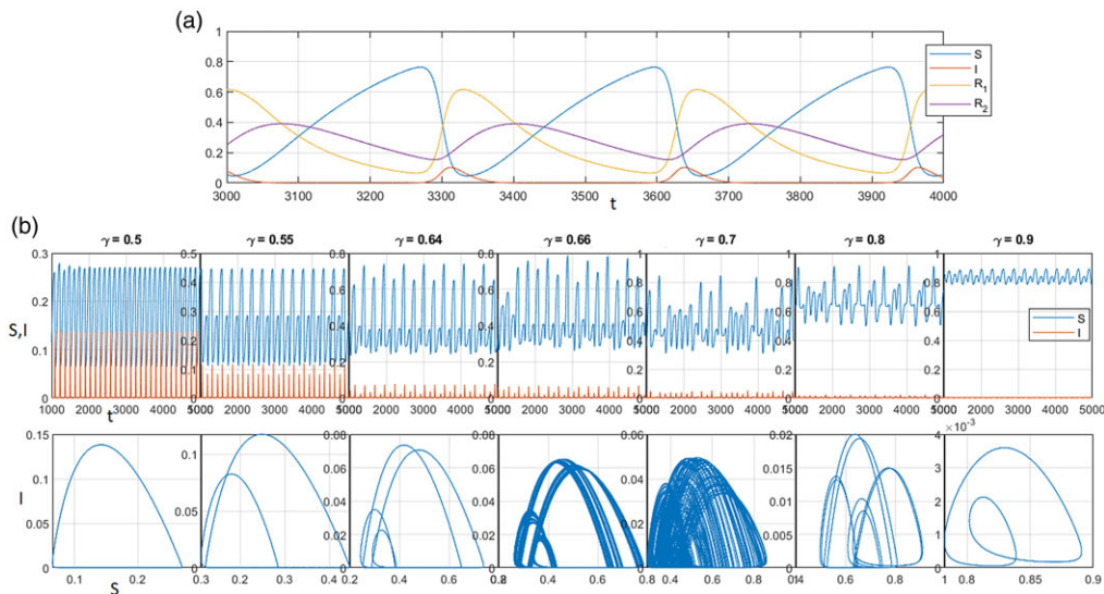
Figure 8. (a) Model (6.4) illustrating sustained persistent outbreaks with n = 2, (\beta_s, \beta_1, \beta_2) = (1, 1, 0), \gamma = 0.7, \mu_1 = \mu_2 = 0.01 . (b) Model (6.4) with \gamma as indicated and other parameters as in (6.5). Note the period-doubling route to chaos.
