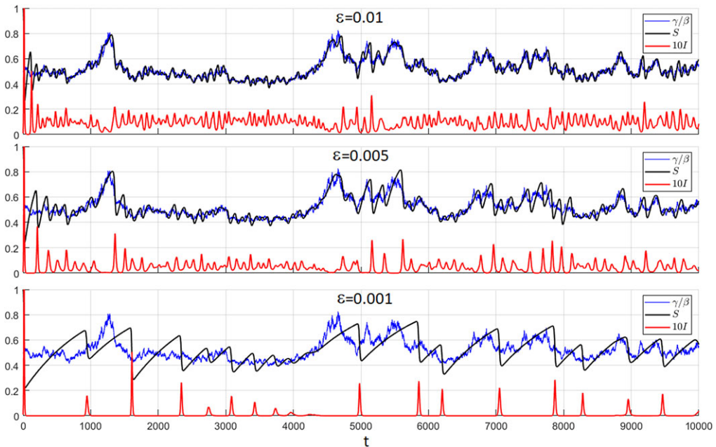
Figure 6. Effect of stochasticity on recurrent outbreaks. Simulation of (2.1) and (6.1) with \beta_0 = 1, \gamma = 0.5, a = 0.001, b = 0.01 and with \varepsilon as indicated. Same stochastic path for \beta was used in all three simulations. Top: the endemic state S ‘follows’ \gamma/\beta without major outbreaks. Middle: decreasing \varepsilon induces some outbreaks. Bottom: even smaller \varepsilon results in recurrent outbreaks.
