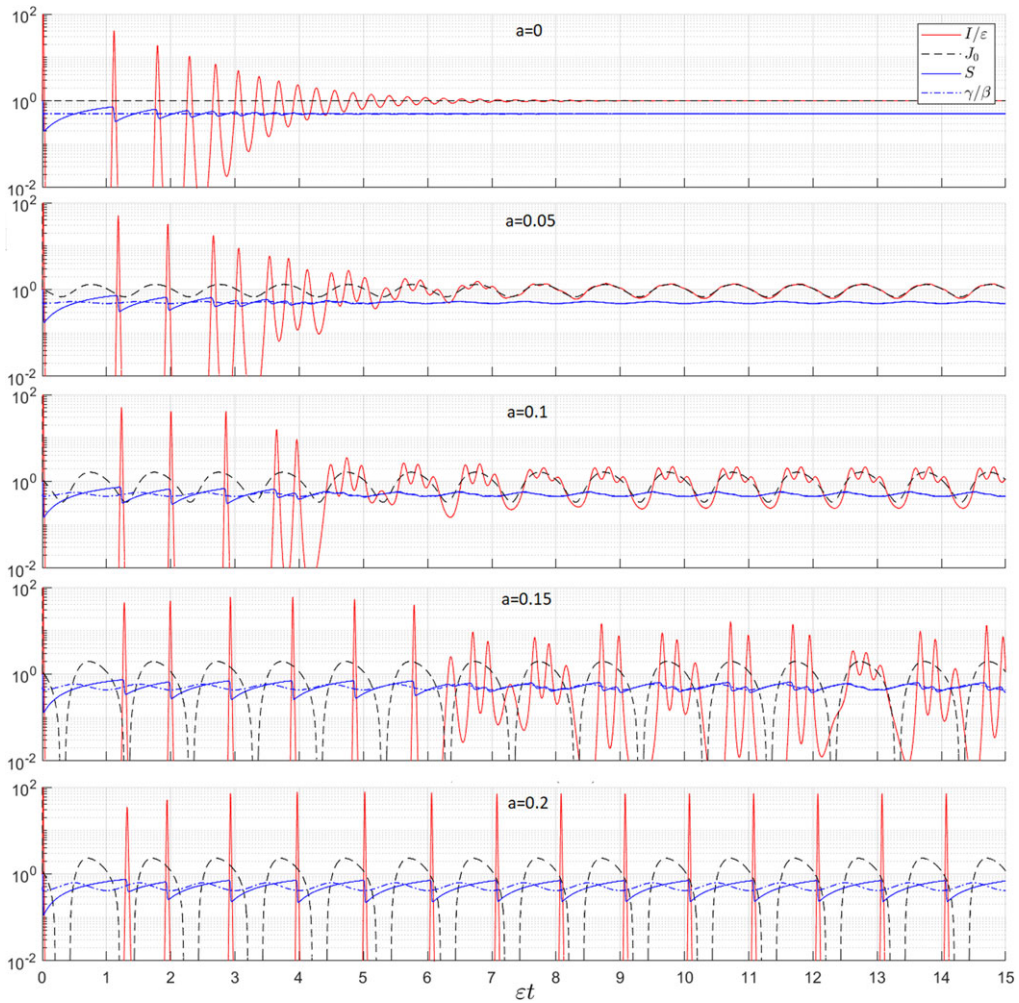
Figure 1. Simulations of (2.1) with \beta(t) = \beta_0 + a \cos(\omega \epsilon t) for several values of a as shown. Other parameters are \beta_0 = 1, \omega = 2\pi, \gamma = 0.5, \epsilon = 0.001 . Initial conditions were taken to be I(0) = 0.01, S(0) = 0.99 . Row 1: constant \beta , damped oscillations towards steady state are observed. Row 2: Convergence towards an adiabatic state. Row 3: Convergence towards adiabatic equilibrium with damped oscillations. Row 4: Onset of small periodic oscillations. Row 5: Large periodic outbreaks. J_0 is defined in (2.7).
